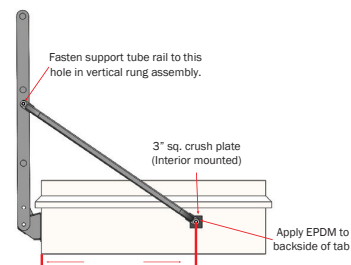
Attach support tubes
