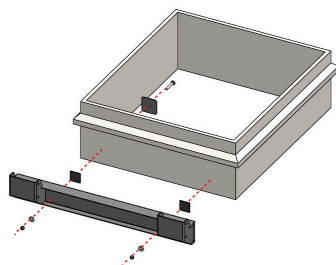
Anchor curb assembly
