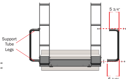
Determine support tube configuration
