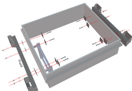
Anchor curb assembly
